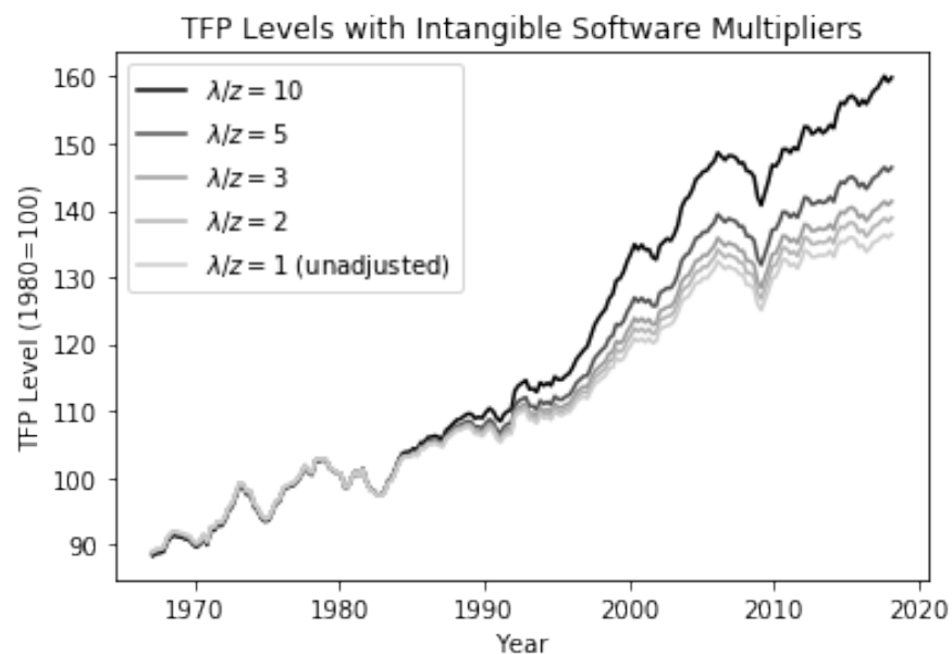
Figure 14: TFP Levels Corrected for Different Software Intangible Multipliers
