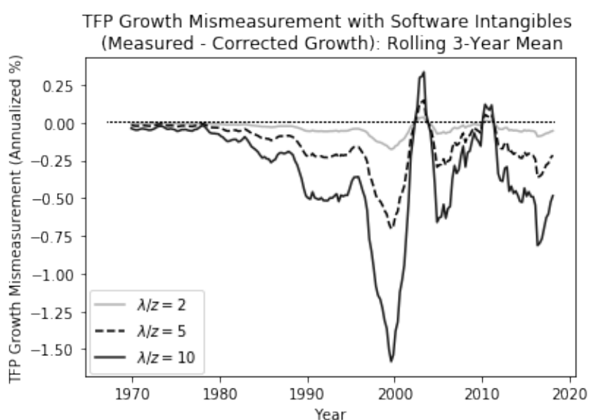
Figure 15: Computer Software-Related TFP Growth Mismeasurement
