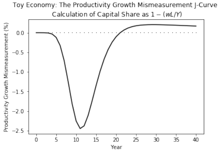
Figure 2: Productivity Growth Mismeasurement with Standard Factor Share Approach
