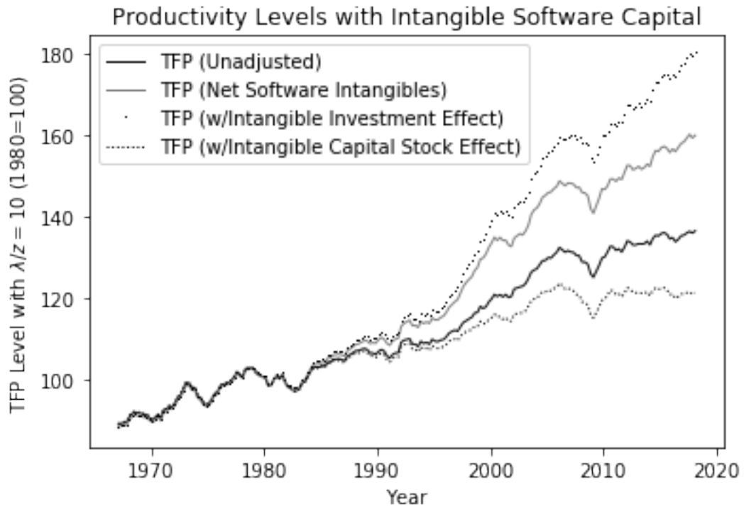
Figure 13: Software-Related Intangible Capital-Adjusted TFP Levels
