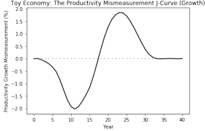
Figure 1: Productivity Growth Mismeasurement with Directly Measured Factor Shares
