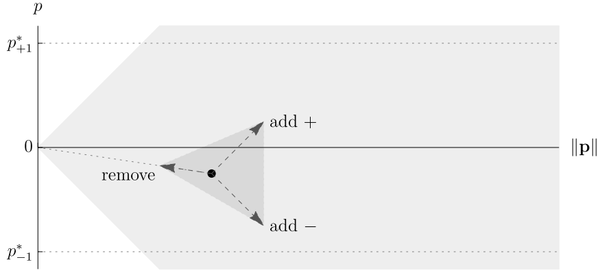
Figure 1: (\frac{d}{dt}\|\mathbf{p}\|, \frac{d}{dt}p) under addition and deletion.
