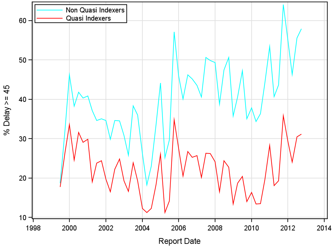
Figure 9. Comparison of time series of excess delay (delay \geq 45 ) between quasi indexer and non quasi indexer institutions: This figure compares the time series of percentage of quasi indexer vs. non quasi indexer institutions that have delays equal to or greater than 45 days in each quarter.
