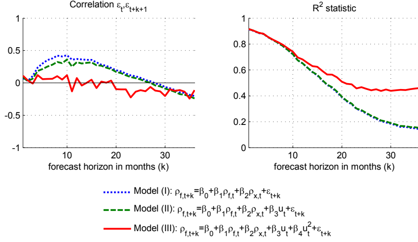
Figure 3: Diagnostic statistics.
