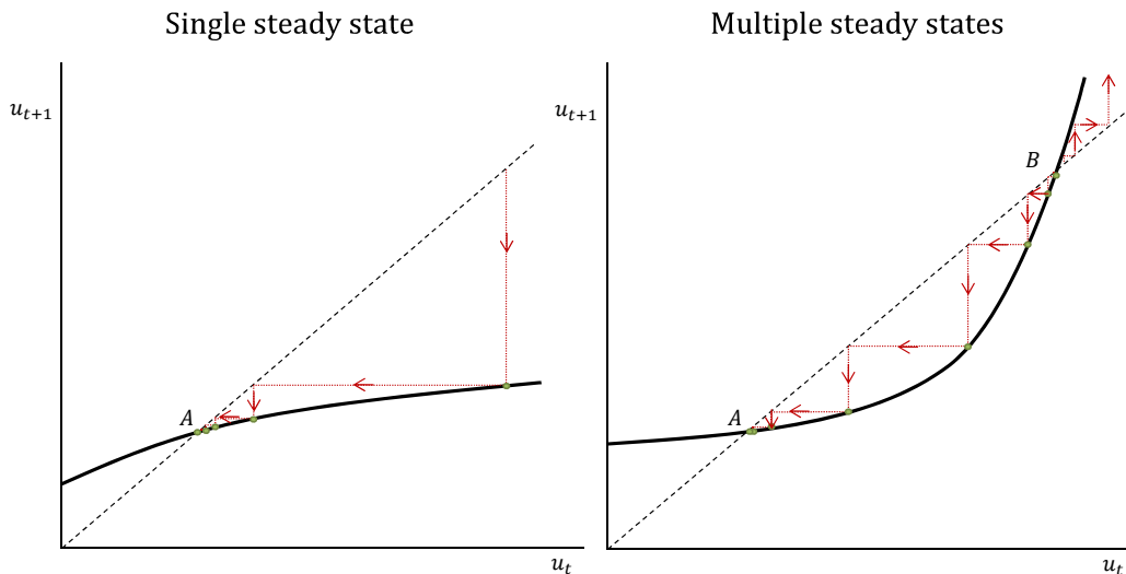
Figure 1: Model illustrations.
